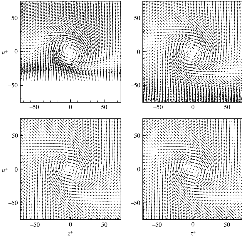
FIGURE 24. Averaged eddy structures in the (\mathbf{e}_z, \mathbf{e}_u) upstream tilted plane at R_\theta = 7500 : y_o^+ = 50, 75, 100 and 125 (clockwise from the top left-hand side).
