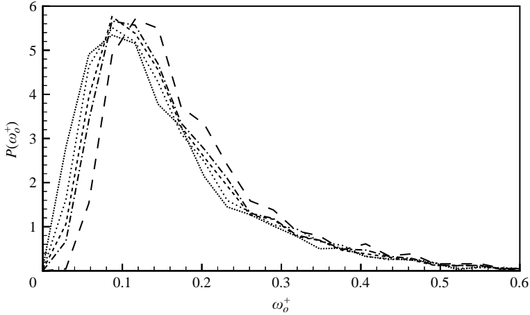
FIGURE 20. Probability density function of \omega_0 in the (e_x, e_y) -plane at R_\theta = 7500 : ..., T = 0.925 , \sigma^+ = 39 ; ···, T = 0.925 , \sigma^+ = 31 ; ---, T = 0.925 , \sigma^+ = 23 ; - - -, T = 0.900 , \sigma^+ = 23 ; - · - ·, T = 0.950 , \sigma^+ = 23 .
