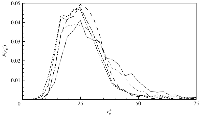
FIGURE 19. Probability density function of r_o in the (\mathbf{e}_x, \mathbf{e}_y) plane at R_\theta = 7500 : \dots , T = 0.925 , \sigma^+ = 39 ; \cdots , T = 0.925 , \sigma^+ = 31 ; -\cdots- , T = 0.925 , \sigma^+ = 23 ; -\cdot-\cdot- , T = 0.900 , \sigma^+ = 23 ; -\cdot-\cdot- , T = 0.950 , \sigma^+ = 23 .
